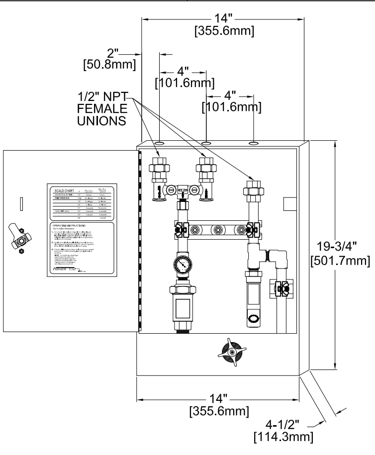
RECESSED MOUNTING
