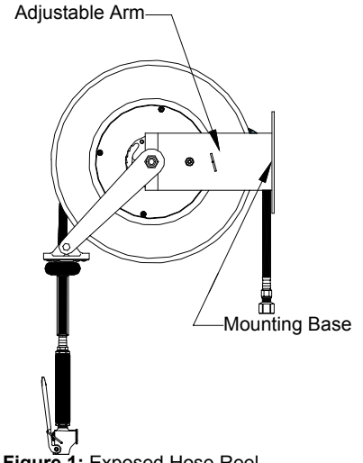
Figure 1: Exposed Hose Reel
