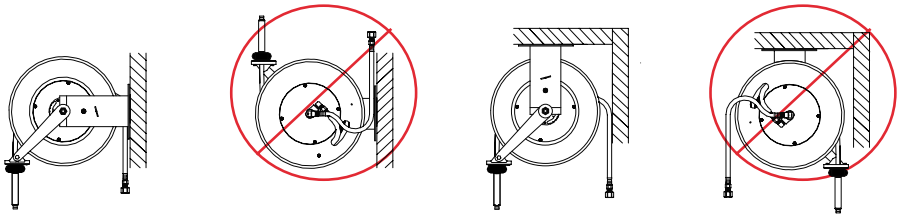
Figure 2: Correct and Incorrect Wall Mounting
